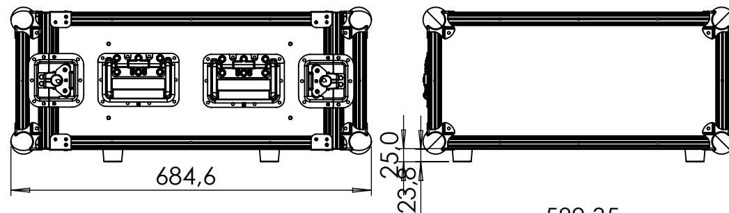
Transport dimensions
